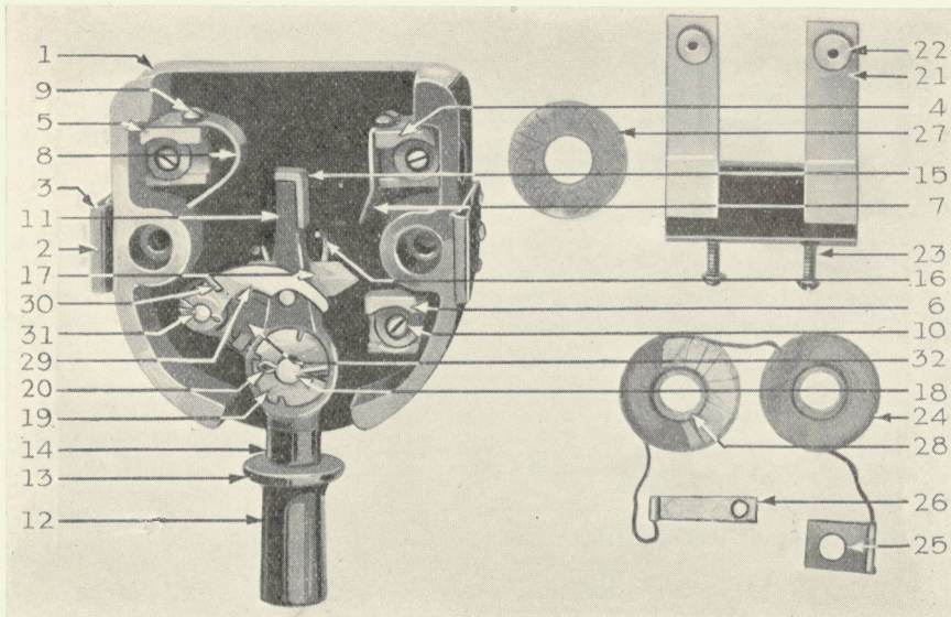
TYPE MS-14 FORM G MAGNETIC BLOWOUT SWITCH
